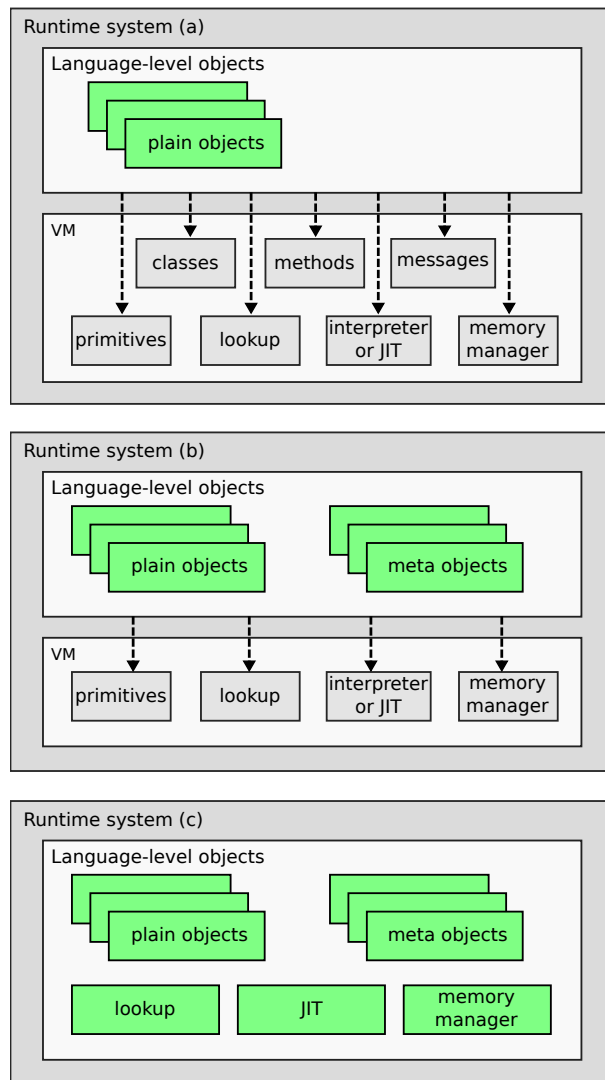
Figure 1. Different interfaces between language and runtime in OO languages, ranging from little or no access (HotSpot), to moderate access (CPython, Squeak) to full access (Bee, Klein)
